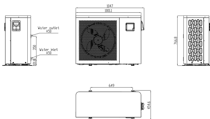
Model : DC E95/E115
